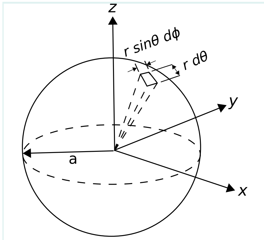
Figure 4.19. Example in spherical coordinates: The area of a sphere.
