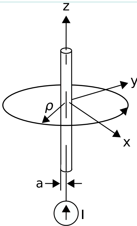
Figure 7.3. Determination of the magnetic field due to steady current in an infinitely-long straight wire.
