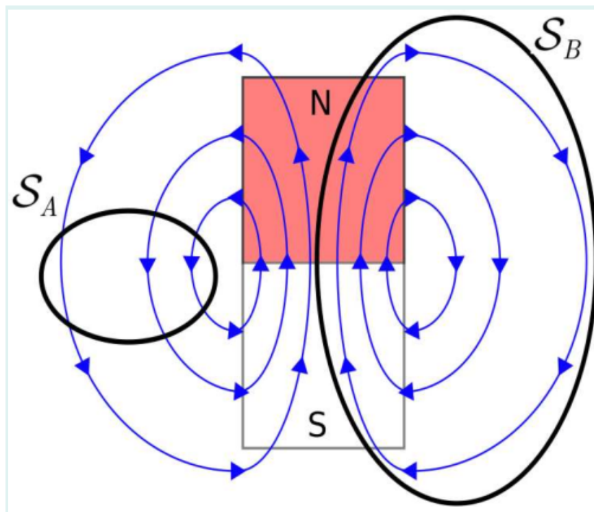
Figure 7.1. Gauss' Law for Magnetostatics applied to a two-dimensional bar magnet. For the surface S = S_A , every field line entering S also leaves S , so the flux through S is
