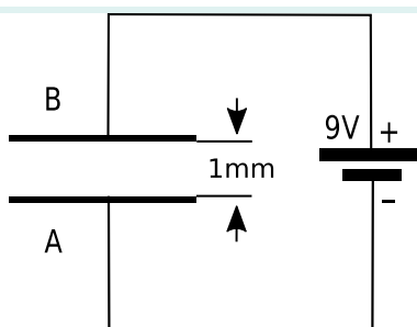
Figure 2.3. A simple circuit used to describe the concept of electric field intensity. In this example, E at point C is 9000 \text{ V/m} directed from B toward A.
