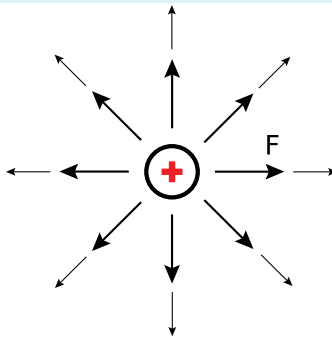
Figure 2.2. A map of the force that would be experienced by a second particle having a positive charge. Here, the magnitude and direction of the force is indicated by the size and direction of the arrow.
