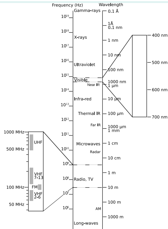
Figure 1.1. Electromagnetic Spectrum.
